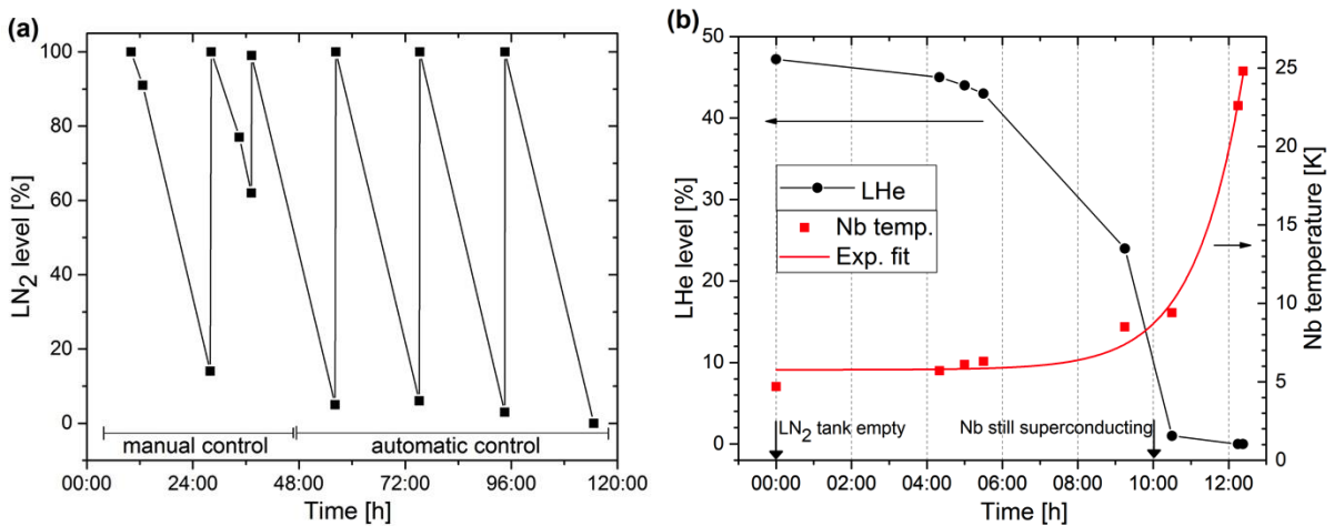
FIG. 11. (a) Automatic refilling of LN 2 in Cryopad on POLI. Manual control is also possible. (b) Warming up of the Cryopad without LN 2 . Solid points are measured values, the red curve is an exponential fit to the temperature data, horizontal arrows indicate corresponding scales and vertical arrows denote times between which the Cryopad remains operational without
