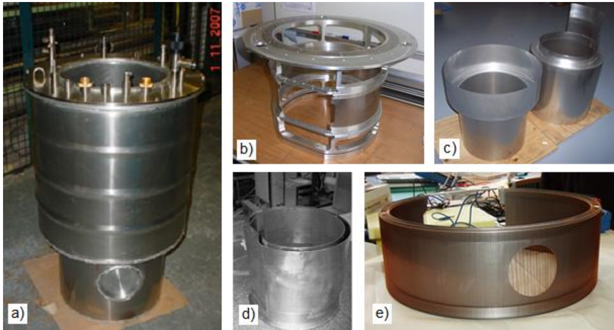
FIG. 1. Main components of the new Cryopad produced by different companies; a) cryostat made by AS Scientific, Oxfordshire, UK, b) precession coils frame made at IFF workshop FZ Jülich, Germany c) \mu -metal shields made by Magnetic Shields Ltd, Kent, UK, d) Nb Meissner screens produced by SDMS, Saint-Romans, France, e) outgoing superconducting precession coil wound at ILL, France.
